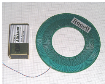
Basic Coil
