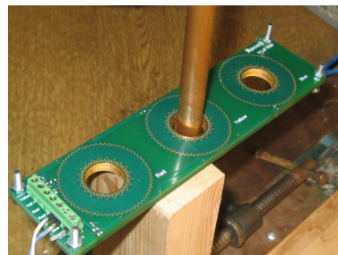
Three-Phase Coil
