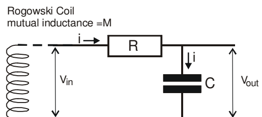
Figure 1: Basic circuit
